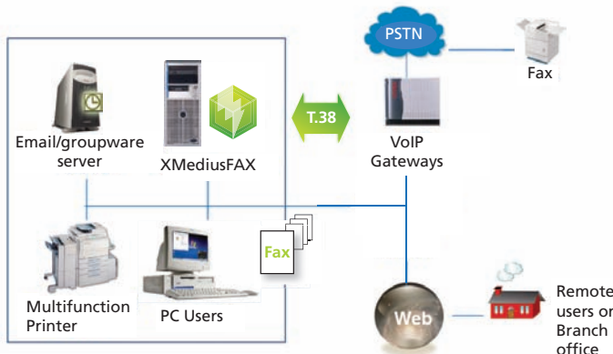
XMEDIUSFAX TYPICAL IMPLEMENTATION
